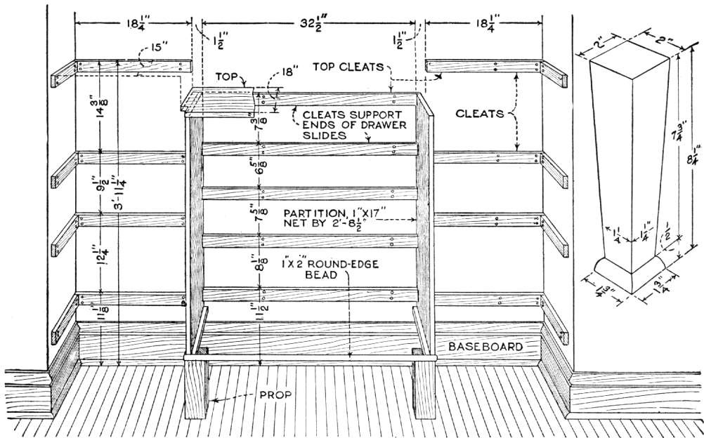
Details of the Shelf and Drawer-Slide Cleats, Nailed to the Wall Studs; Partitions in Place Ready for the Frames, and Detail of Legs
